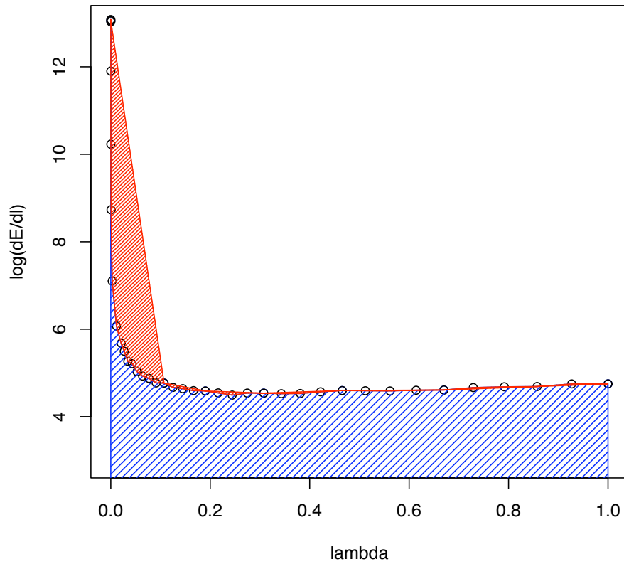
Figure 11: Sample TI data ( \log(\langle \frac{\partial U}{\partial \lambda} \rangle) ) against \lambda . The blue shaded area shows the integral with fine sampling close to the end point. The red area shows the difference when \lambda values are more sparse. In this example, insufficient sampling before \lambda \simeq 0.1 can result in a large overestimation of the integral. Beyond \simeq 0.2 , sparser sampling is justified as dE/d\lambda is not changing quickly.
