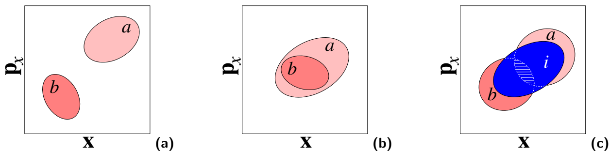
Figure 9: Convergence of an FEP calculation. If the ensembles representative of states a and b are too disparate, equation (29) will not converge (a) . If, in sharp contrast, the configurations of state b form a subset of the ensemble of configurations characteristic of state a , the simulation is expected to converge (b) . The difficulties reflected in case (a) may be alleviated by the introduction of mutually overlapping intermediate states that connect a to b (c) . It should be mentioned that in practice, the kinetic contribution, \mathcal{T}(\mathbf{p}_x) , is assumed to be identical for state a and state b .
