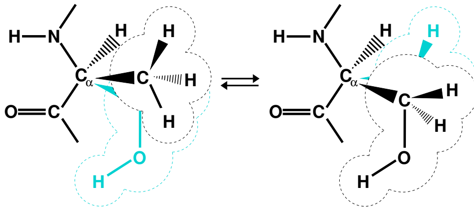
Figure 8: Dual topology description for an alchemical simulation. Case example of the mutation of alanine into serine. The lighter color denotes the non-interacting, alternate state.
