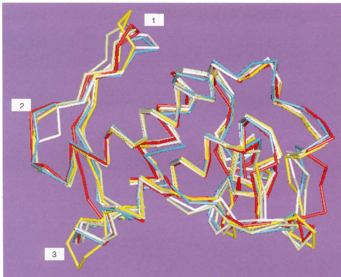
Fig. 6. Comparison of the averaged structure obtained from simulation T , simulation L and simulation A with the crystal structures reported in Scott et al. 14 and Wery et al. 13 ; only protein C α atoms are presented. White, structure reported in Scott et al. 14 ; yellow, structure reported in Wery et al. 13 ; red, averaged MD structure from simulation T , blue, averaged MD structure from simulation L ;
