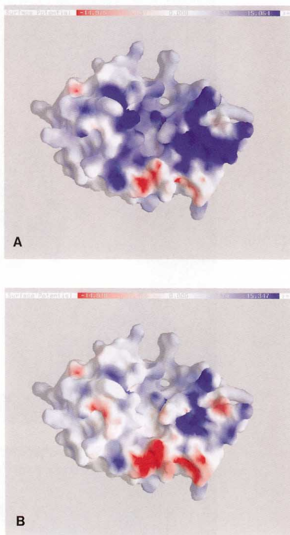
Fig. 9. Electrostatic potential on the \text{PLA}_2 surface for an enzyme-protein complex taken from simulation T at 120 ps. The potential shown is in units of k_B T/e . A : \text{PLA}_2 associated with a neutral membrane surface. B : \text{PLA}_2 associated with a negatively charged membrane surface, with a total charge per lipid of -0.1 e .
