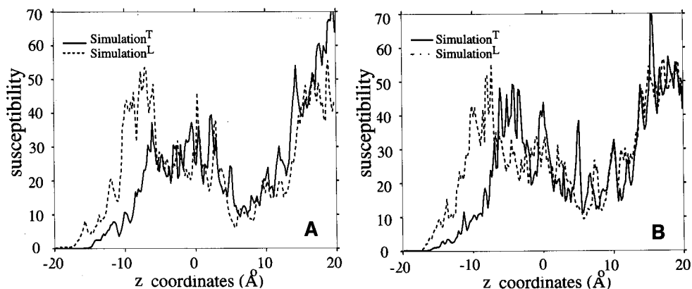
Fig. 5. Dielectric susceptibility along the z-axis in the protein-membrane interface calculated from simulation T and simulation L . A: Atoms within a radius of 10.0 Å around the z-axis are included. B: Atoms within a radius of 15.0 Å around the z-axis are included.
