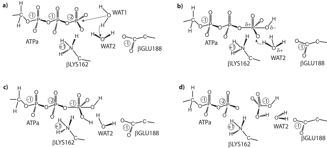
Figure 2: Schematic representation of the multi-center reaction for ATP hydrolysis, showing the a) reactant, b) transition, c) intermediate and d) product state. (Figure reprinted with permission from Dittrich et al. (2003). Copyright 2003 Biophysical Society.)
