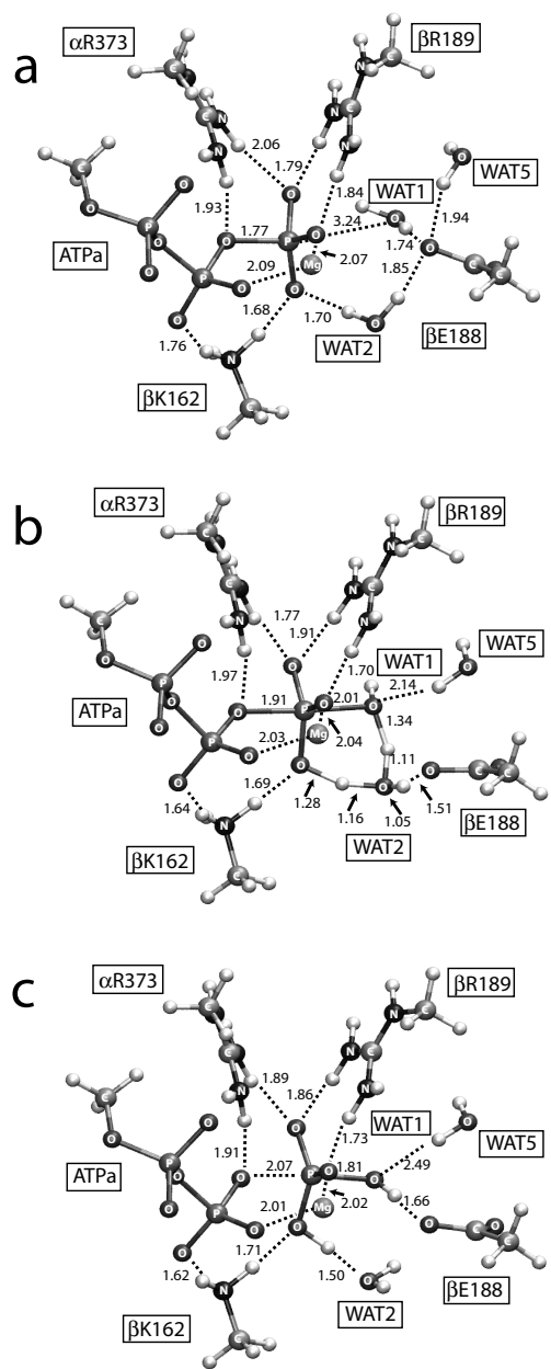
Figure 1: ATP hydrolysis reaction in the \beta_{DP} catalytic site. Shown are the reactant ( a ), transition ( b ), and final ( c ) state conformations. In ( b ) the involvement of two water molecules is clearly discernible in the form of an intermediate H_3O^+ -like construct. (Figure adapted with permission from Dittrich et al. (2004). Copyright 2004 Biophysical Society.)
