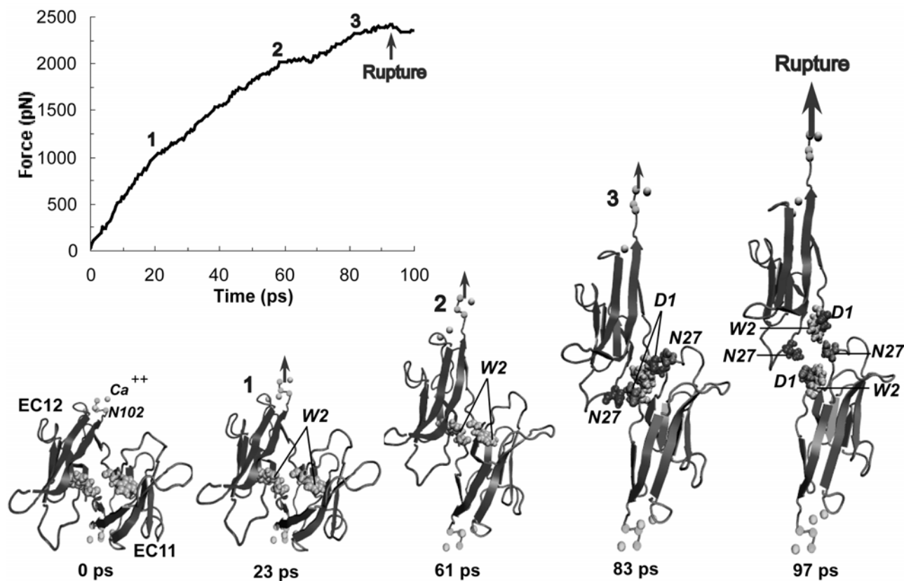
Figure 3 : Snapshots of the complex during one of the simulations performed at 1\text{\AA}/\text{ps} . The inset shows the corresponding force-extension profile. The rupture process is mainly characterized by the extraction of the conserved tryptophan side chains from their pockets.
