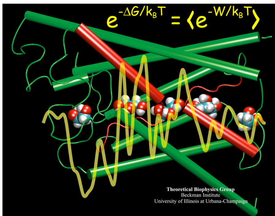
Free Energy of Glycerol Transport
