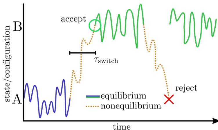
Figure 13: The basic constant-pH MD scheme in NAMD is to alternate equilibrium sampling in a fixed protonation state followed by a nonequilibrium MD Monte Carlo move to sample other protonation states. The latter move can be accepted or rejected. If accepted, the simulation continues in the new protonation state. If the move is rejected, sampling continues as if the move were never attempted at all.
