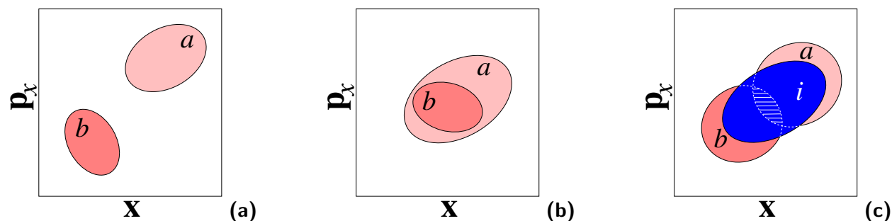
Figure 7: Convergence of an FEP calculation. If the ensembles representative of states a and b are too disparate, equation (77) will not converge (a). If, in sharp contrast, the configurations of state b form a subset of the ensemble of configurations characteristic of state a , the simulation is expected to converge (b). The difficulties reflected in case (a) may be alleviated by the introduction of mutually overlapping intermediate states that connect a to b (c). It should be mentioned that in practice, the kinetic contribution, \mathcal{T}(\mathbf{p}_x) , is assumed to be identical for state a and state b .
