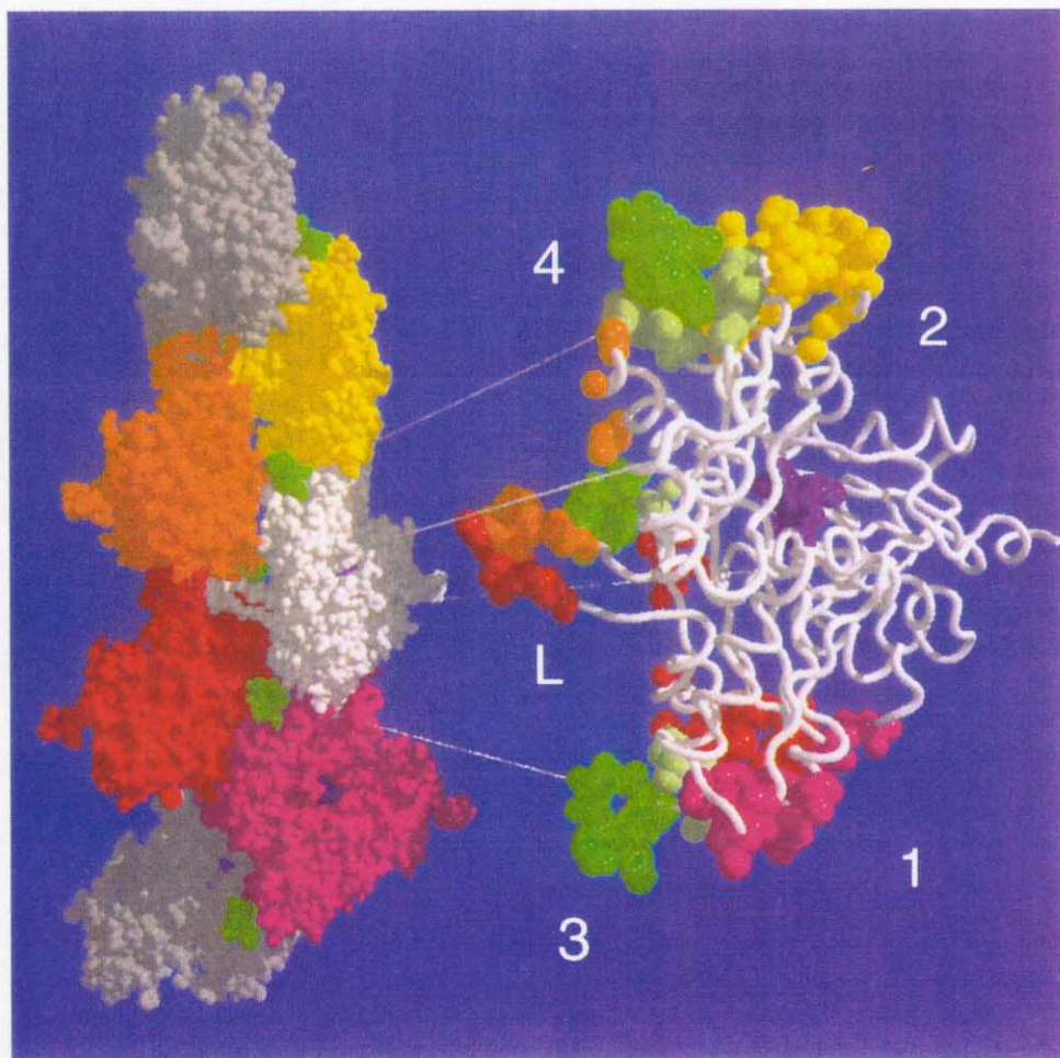
FIGURE 1 Lorenz F-actin model with phalloidin (Lorenz et al., 1993) ( left ) and contact regions in the monomer ( right ), visualized by Radiance (Ward, 1994). Phalloidin peptides are shown in green, ADP nucleotides in purple. The enlarged monomer highlights interactin contacts and actin-phalloidin contacts ( solid sphere representation ). The color of the spheres codes for the neighboring monomer or phalloidin in the filament ( left ). Of special interest is the hydrophobic plug loop (L), which connects the two strands of the filament by interacting with two opposing monomers ( red, orange ). Each phalloidin molecule interacts with three actin monomers. The indices 1–4 identify actin's structural subdomains.
