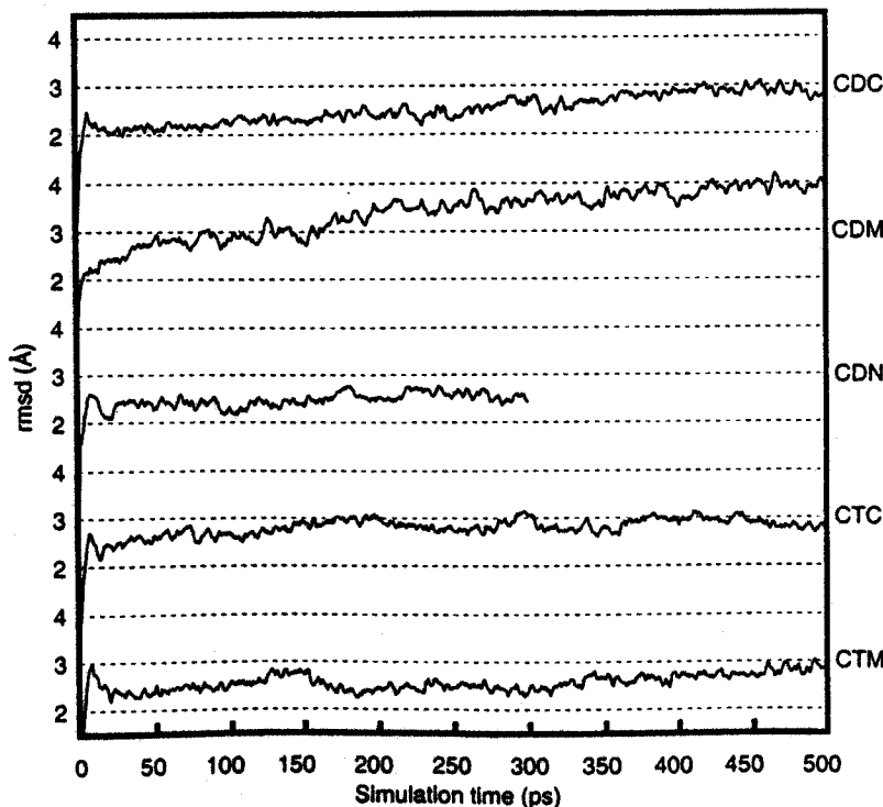
FIGURE 2 Backbone rms deviations from the respective initial structures as a function of simulation time. Deviations of the trajectories CDC, CDM, CDN, CTC, and CTM are compared.
