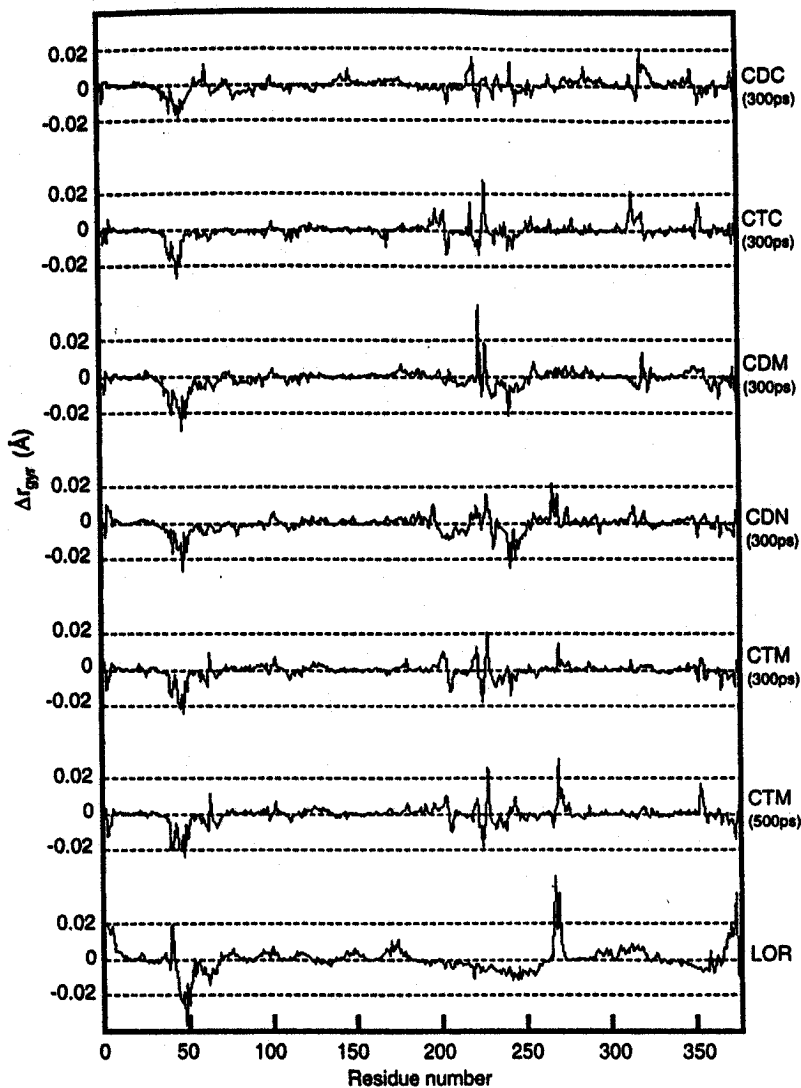
FIGURE 9 First-order contributions to differences in radius of gyration, \Delta r_{\text{gyr}} , of residues from simulated structures and from the Lorenz F-actin model relative to the Kabsch crystal structure (KAD). The contributions from Eq. 4 have been summed up for each residue. For simulated structures, the simulation time is indicated.
