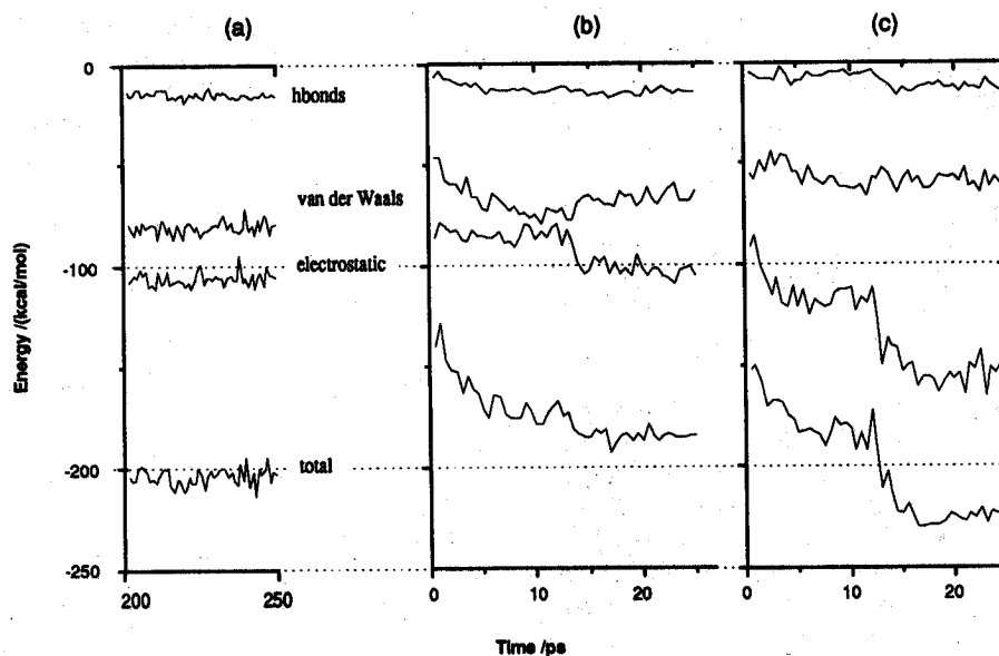
FIGURE 8: Comparison of the nonbonded energies between the DNA helix and distamycin during the latter part of the 250-ps simulation (a), during reentry into the minor groove (b), and in the major groove (c).
